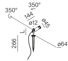
DART LED exterior upright
