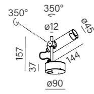
DART LED exterior spot
