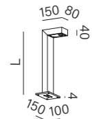
SLUP LED exterior upright
