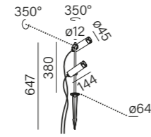
DARTx2 LED exterior upright
