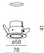
PUTT mini LED recessed
