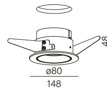
PUTT midi LED recessed
