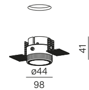
PUTT mini LED trimless recessed
