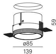
PUTT maxi LED trimless recessed
