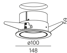
PUTT maxi LED recessed
