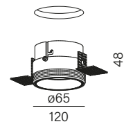
PUTT midi LED trimless recessed
